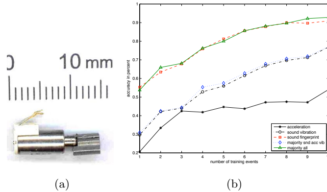
Fig. 3: A common vibration motor 2 (Figure (a)). On the right (b) is the Classification accuracy depending on the number of training events for the office scenario depicted.
